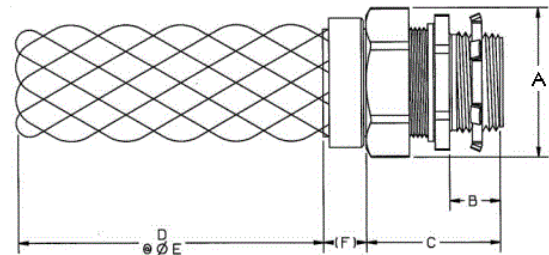
STRAIGHT INSULATED
